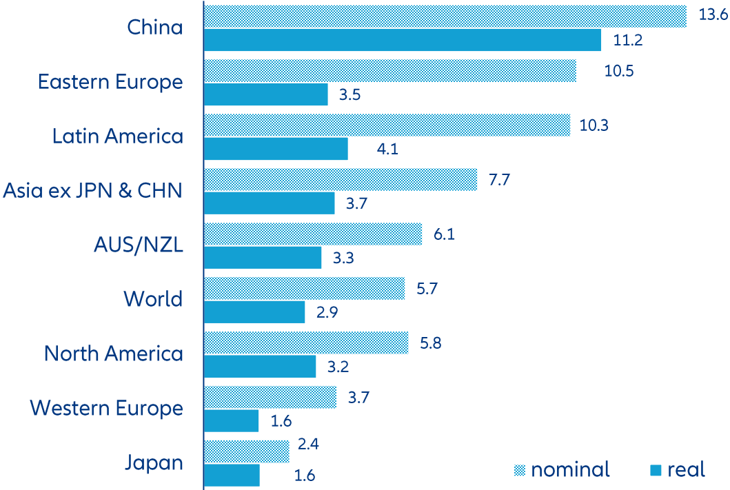
Growth of net financial assets per capita CAGR* 2006 to 2025, nominal and real, in %
