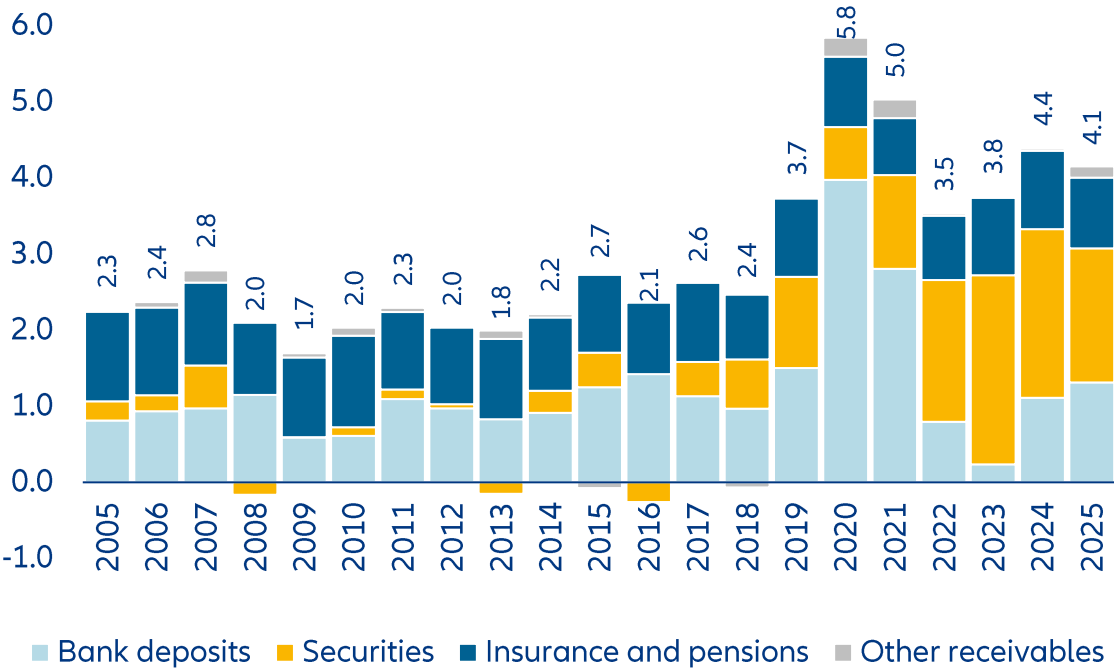
Net acquisition of financial assets by asset class in 2025 EUR trillion
